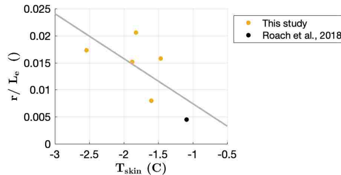
Figure 2.11: Average floe radius, scaled by wavelength, as a function of skin temperature. Yellow points are from this study, and black point is from Roach et al. [2018b]. R^2 = 0.45
