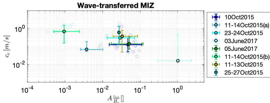
Figure 4.11: Effective transfer velocity in wave-transferred MIZ using the results of Fig. 4.9, as a function of ice concentration and nondimensional ice thickness ( A \frac{z_{ice}}{H_s} ). Each color represents a deployment in the wave-transferred MIZ.
