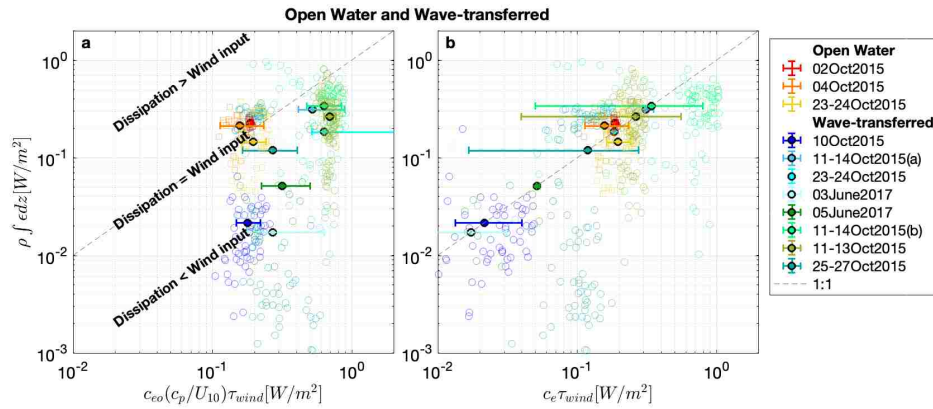
Figure 4.9: (a) Comparison of vertically integrated TKE dissipation rates with input rate from wind expected based on open water conditions. (b) The same comparison where input rate for the wave-transferred MIZ uses effective transfer velocities determined assuming a balance of wind input and observed dissipation rates. Each color represents a SWIFT deployment (warm colors represent open water, and cool colors represent wave-transferred MIZ), and filled points represent averages for each deployment. Bars represent the range of measured drag coefficients, when applicable. Dashed black line is the 1:1 line, where expected input and dissipation are equal. Wave-transferred MIZ bin-averages in (b) have been forced to lie on the line.
